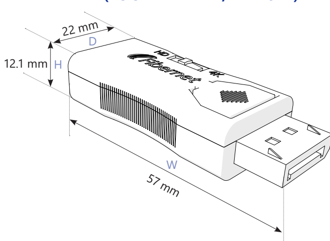
MyBlocker – DisplayPort Input (FIS-SVID-11DP-4K/FHD Rev B)
